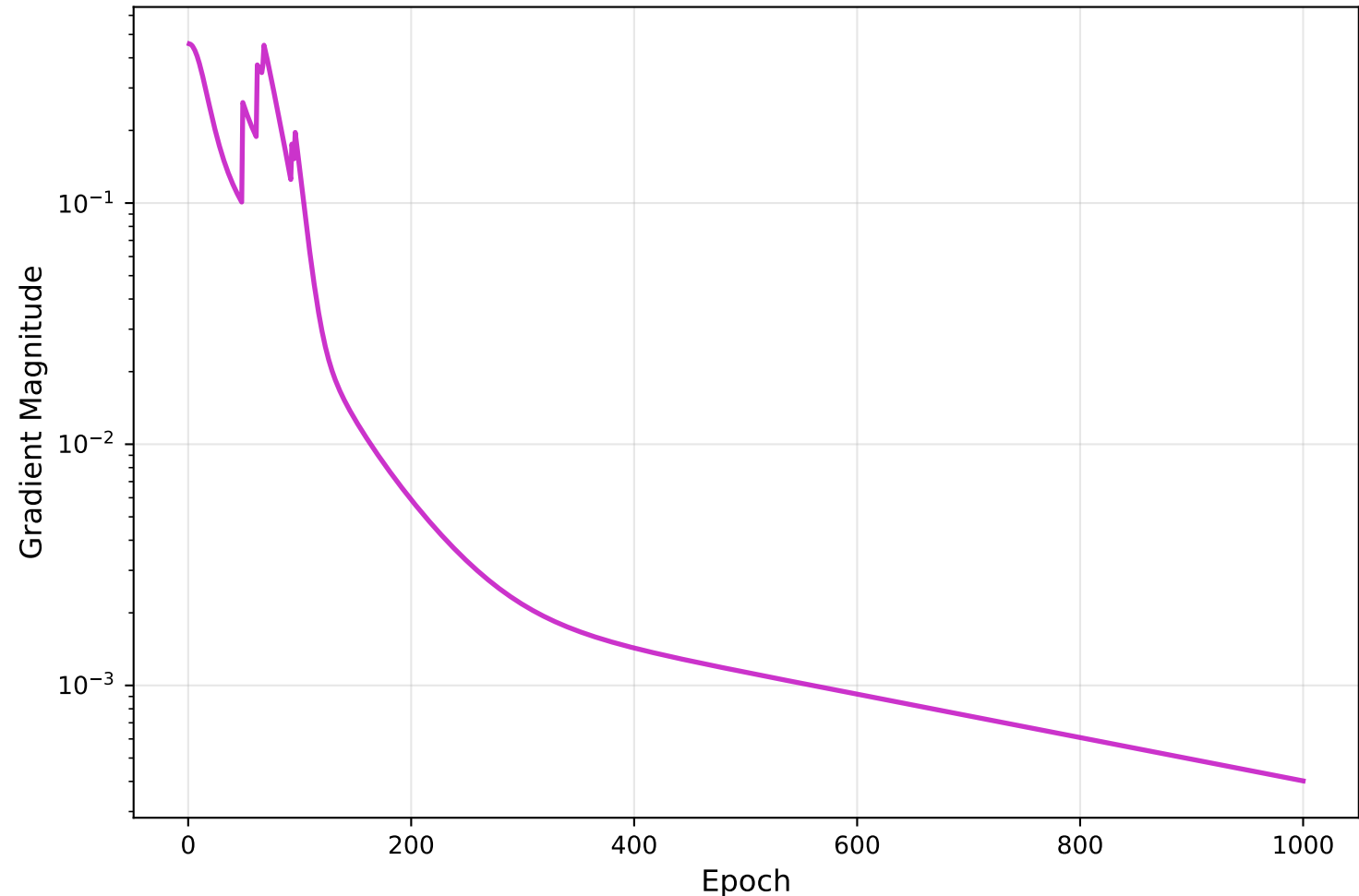
Gradient Evolution (Log Scale)
